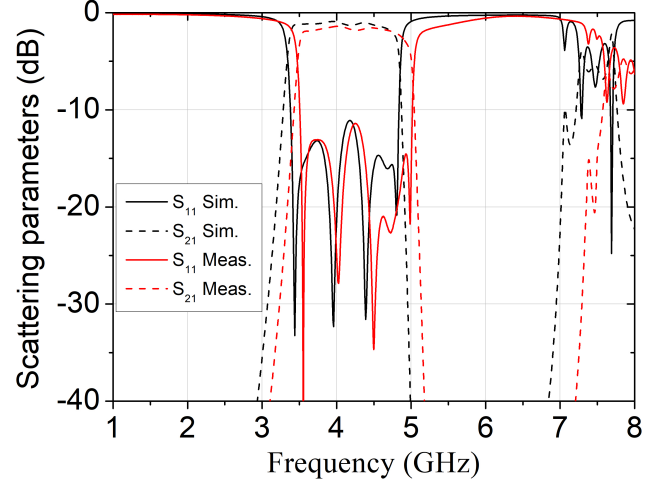
Fig. 8. Simulated and measured S-parameters of the glide-symmetric air-filled periodic SIW filter of Fig. 7.
